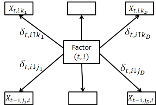
Figure 2: Factor for MPLP based HO Matching
