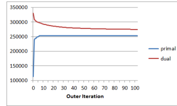
Figure 4: Change in primal and dual during MPLP iterations on PSU Seq 3
