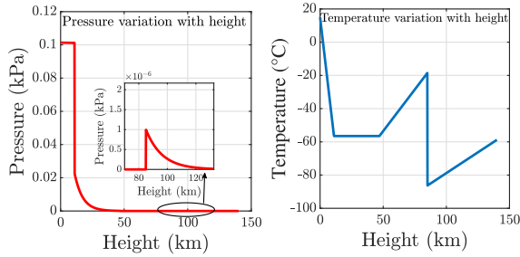
Fig. 2. Pressure and temperature variation with height based on the U.S. Standard Atmosphere, 1976 [40].
