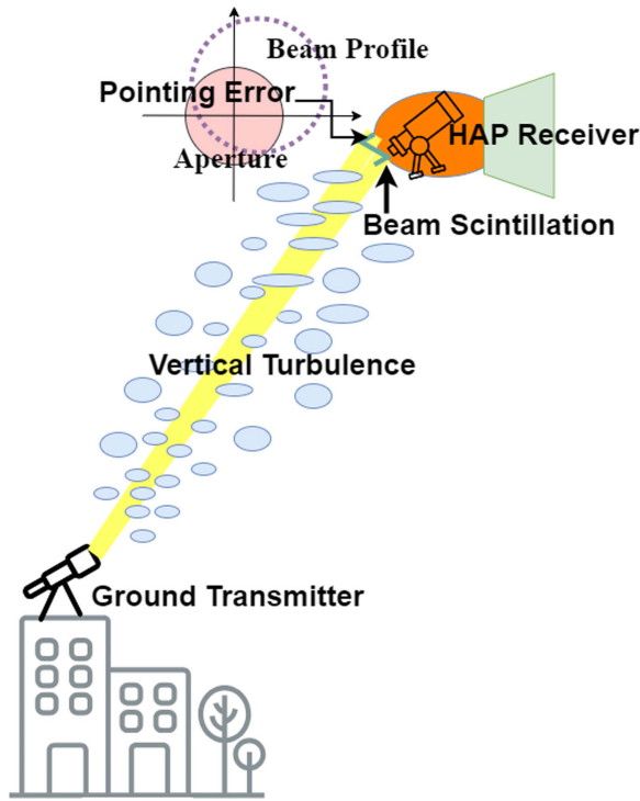
Fig. 1. Ground-HAP FSO system model affected by vertical turbulence.
