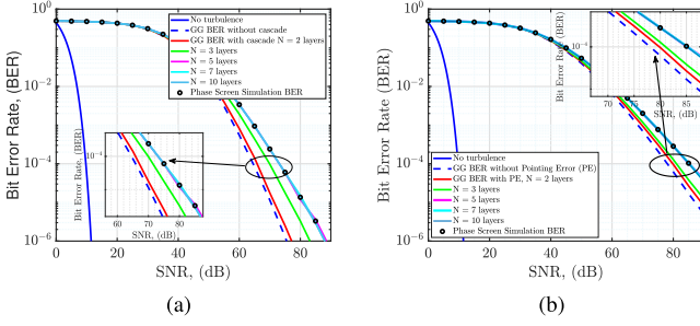
Fig. 9. (a) Average BER performance of concatenated gamma-gamma (GG) turbulence channel. Correlated phase screen based simulation results are denoted by circles. (b) Average BER performance of cascaded GG turbulence channel by considering composite effect of turbulence and pointing errors.
