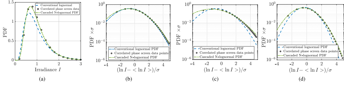
Fig. 6. Scaled log-irradiance PDF for a plane optical beam travelling in weak turbulence regions in vertical FSO link configuration ( \epsilon = 10\% and l_o/R_F = 0.5 ) (a) Vertical link distance = 10 km (Linear Scale) (b) Vertical link distance = 10 km (logarithmic scale) (c) Vertical link distance = 15 km (logarithmic scale) (d) Vertical link distance = 25 km (logarithmic scale).
