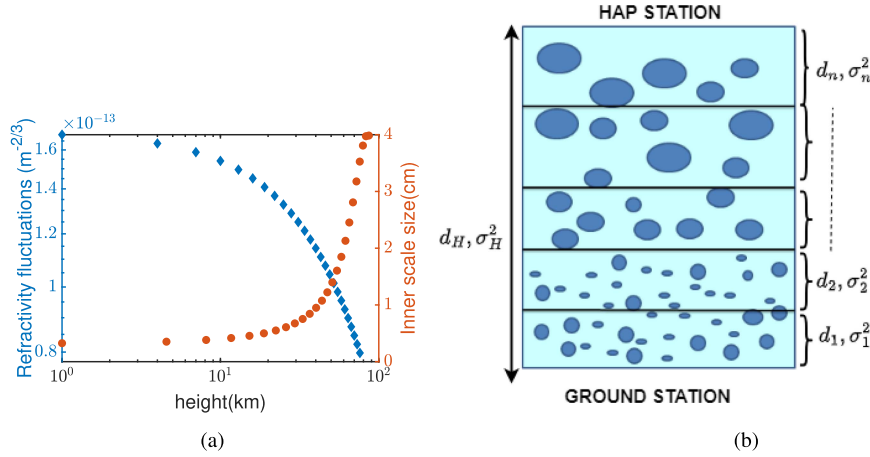
Fig. 3. Illustration of (a) Refractive index and eddy size variation versus height; (b) HAP-based VFSO network.
