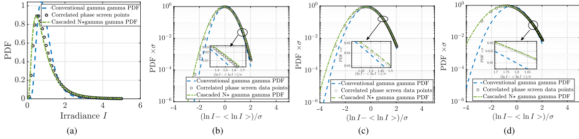
Fig. 7. Scaled log-irradiance PDF for a plane optical beam traveling in very strong turbulence regions in vertical FSO link configuration ( \epsilon = 10\% and l_o/R_F = 0.5 ) (a) Vertical link distance = 10 km (Linear Scale) (b) Vertical link distance = 10 km (logarithmic scale) (c) Vertical link distance = 15 km (logarithmic scale) (d) Vertical link distance = 25 km (logarithmic scale).
