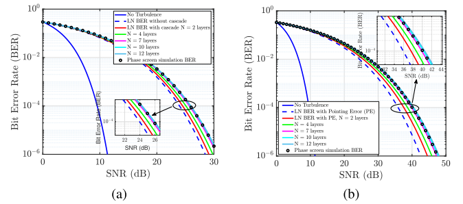
Fig. 8. (a) Average BER performance of cascaded lognormal (LN) turbulence channel by considering different number of layers. Correlated phase screen based simulation results are denoted by circles. (b) Average BER performance of cascaded lognormal turbulence channel by considering composite effect of turbulence and pointing errors.
