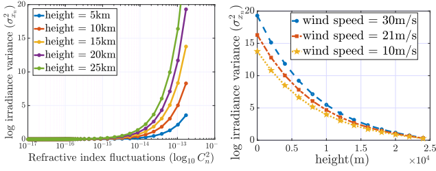
Fig. 5. Variation in log-irradiance values with changes in height and variations in the refractive index structure parameter as one ascends from ground level.
