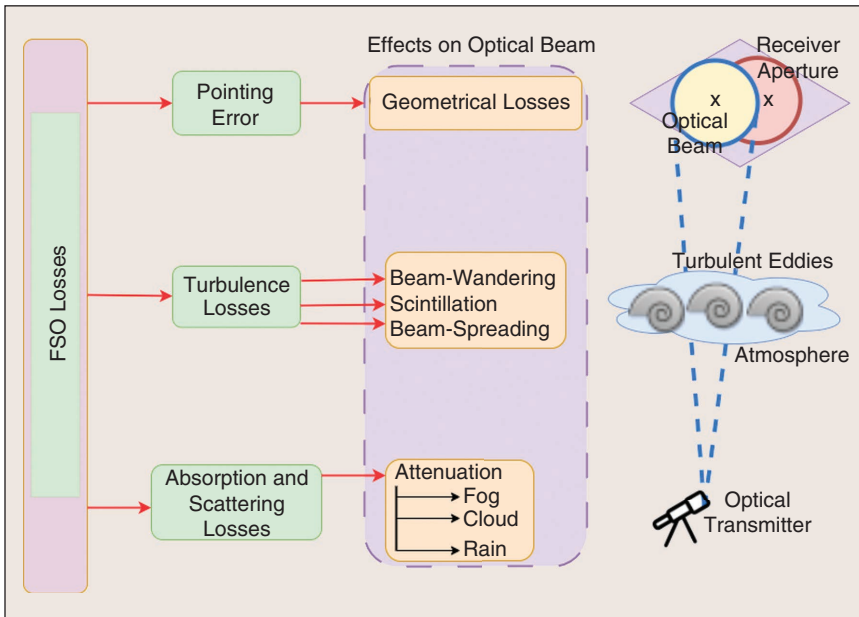
FIGURE 3 FSO channel induced losses faced by optical beam. Turbulence-induced beam-spreading and beam-wandering dominate in good weather conditions.
