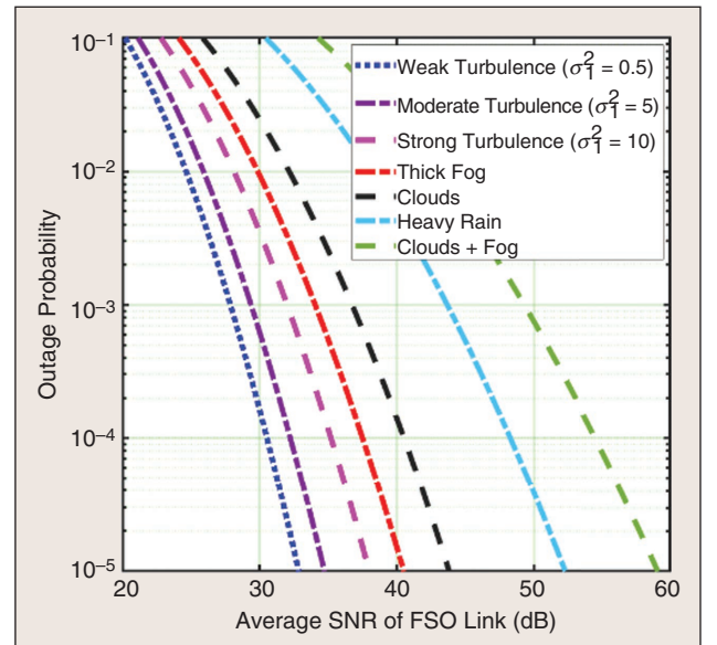
FIGURE 4 Outage probability versus average SNR.
