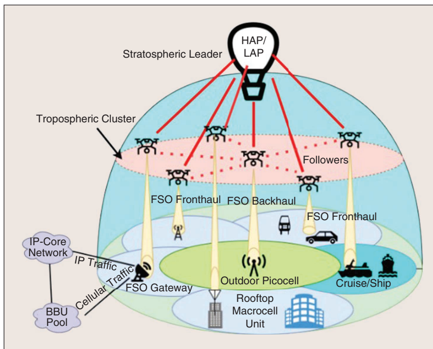
FIGURE 2 The conceptual topology of vertical fronthaul/backhaul FSO framework for 6G wireless networks.
