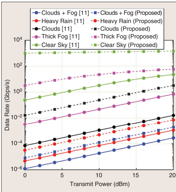
FIGURE 6 Data rate versus transmit power.
