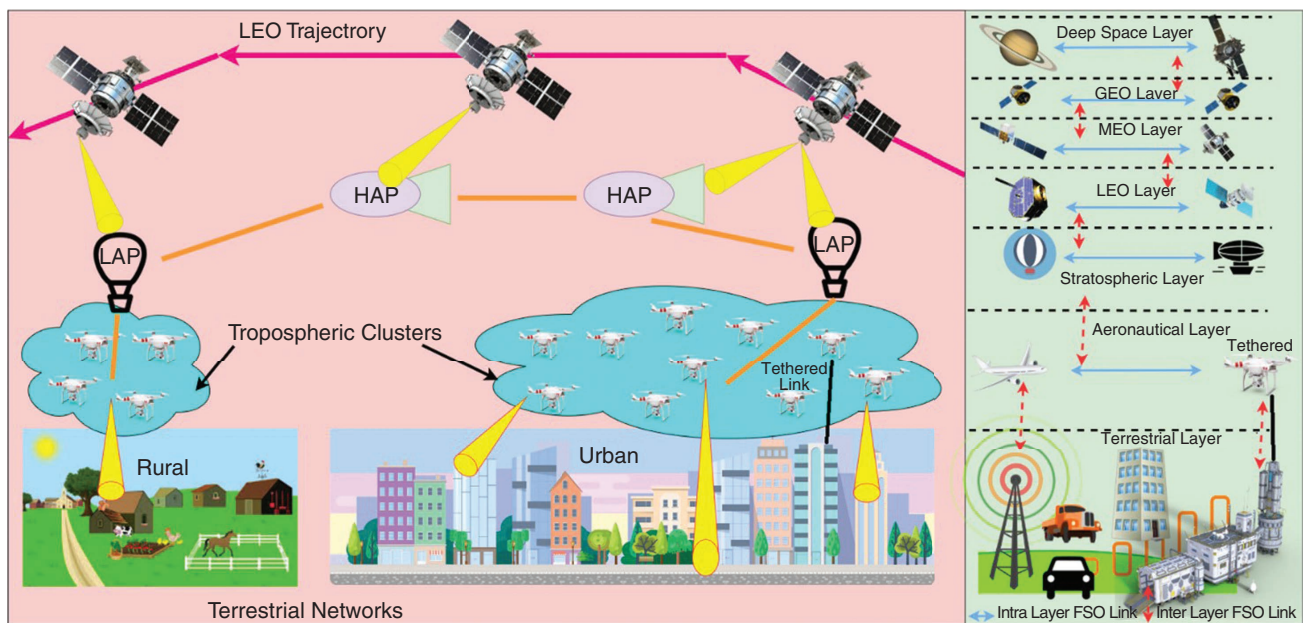
FIGURE 1 A generic SAGIN architecture, with layers at different altitudes: deep space ( >35,838 km), GEO (12,000–35,838 km), medium Earth orbit (2,000–12,000 km), LEO (200–2,000 km), stratospheric (17–22 km), and aeronautical (0.15–17 km) layer. Stratospheric platforms help in mitigating zenith angle limitations for satellite-to-ground FSO links and managing coordinated tropospheric clusters.
