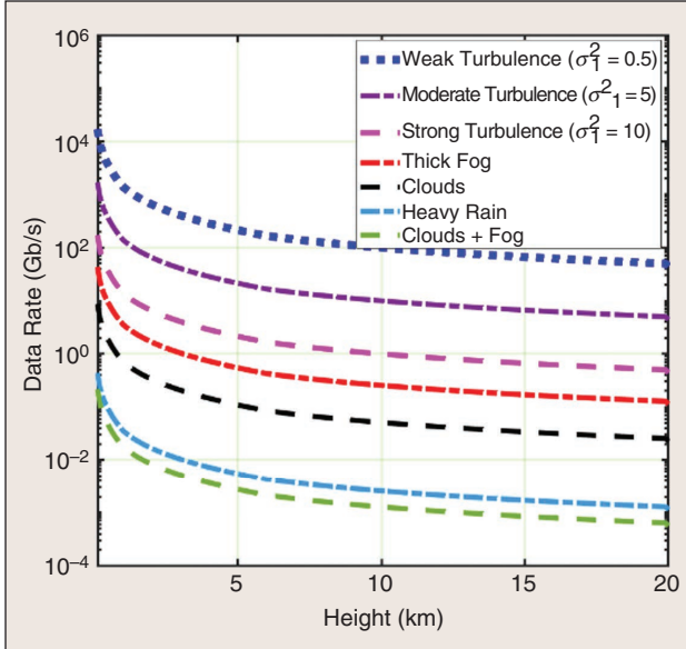
FIGURE 5 Data rate versus aerial platforms height.
