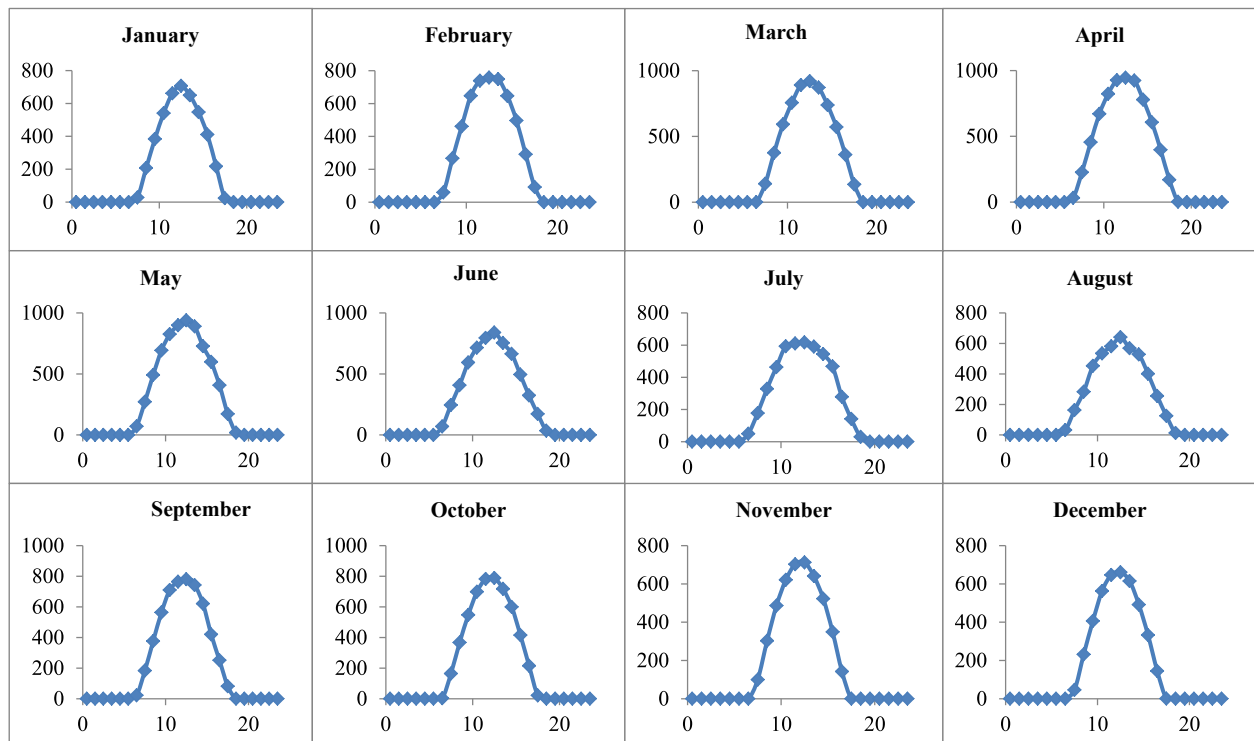
Fig. 15. Solar irradiance in Munnar, Kerala, India [x-axis represents the time in hrs; y-axis represents the solar irradiance data in \text{W/m}^2 ] [74].
