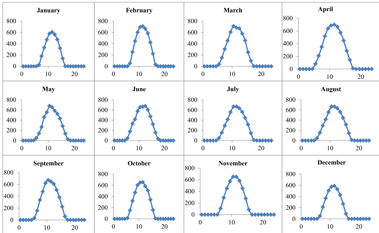
Fig. 14. Solar irradiance in Golaghat, Assam, India [x-axis represents the time in hrs; y-axis represents the solar irradiance data in \text{W/m}^2 ] [74].
