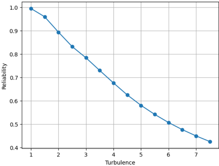
Figure 14: Reliability values at different turbulence levels
