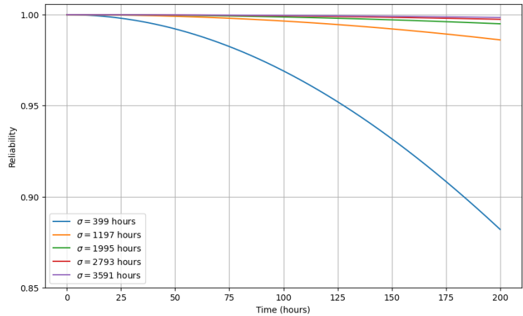
Figure 8: Reliability of laser subsystem for Rayleigh distribution
