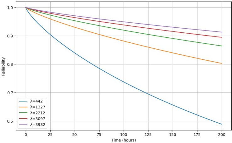
Figure 4: Reliability of laser subsystem for Weibull distribution ( k = 0.8 )
