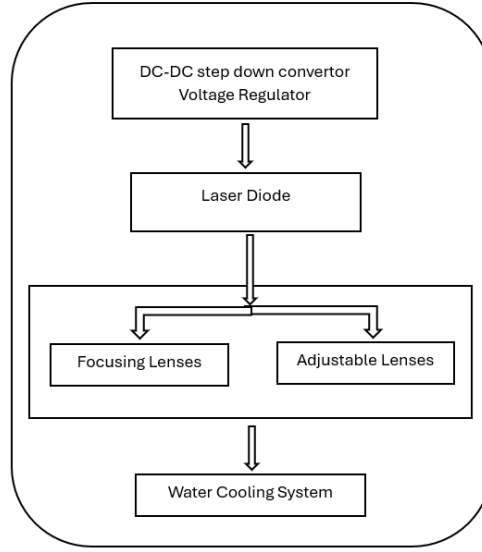
Figure 3: Block Diagram of Laser System
