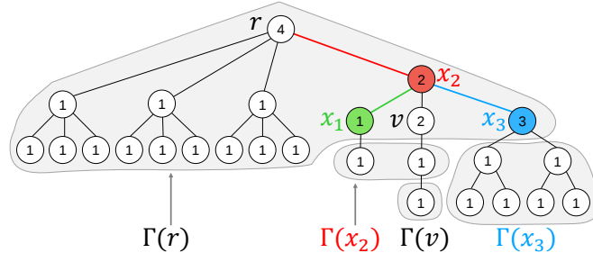
■ Figure 2 Tree MINND-realization of \sigma = (4^1 3^1 2^2 1^{22}) . The number in each vertex denotes its MINND. The edges (y_1, x_1) , (y_2, x_2) and (y_3, x_3) are colored green, red and blue, respectively. Further, A = \{x_3\} and B = \{x_1, x_2\} .
