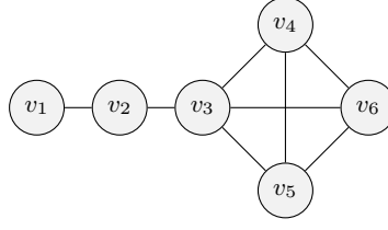
■ Figure 4 MINND-realization of sequence \sigma = (3^3 2^1 1^2) . Here \text{MINND}(v_1) = \text{MINND}(v_2) = \deg(v_1) = 1 , \text{MINND}(v_3) = \deg(v_2) = 2 , and \text{MINND}(v_i) = 3 , for i \in \{4, 5, 6\} . Since \text{leader}(v_2) = v_1 and \text{leader}(v_3) = v_2 , thus, v_2 is a leader as well as a follower.
