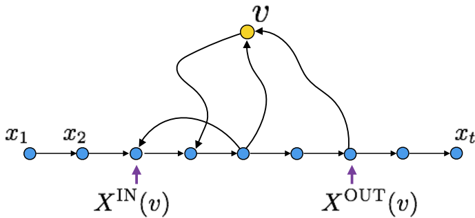
Fig. 2 Depiction of X^{\text{IN}}(v) and X^{\text{OUT}}(v) for a vertex v whose SCC intersects X
