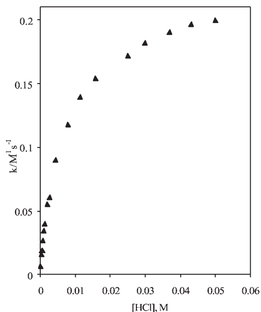
Figure 1. A specific acid-catalyzed Diels–Alder reaction profile for 1b with 2 at 32 °C
