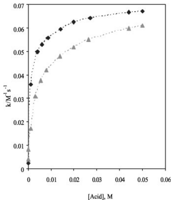
Figure 3. A reaction profile of the reaction of dienophile 1a with cyclopentadiene 2 in DCI (◆) and HCl (▲) at 32 °C to establish k_H/k_D
