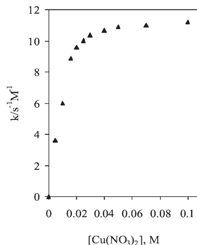
Figure 2. Copper(II) nitrate catalysis of the Diels–Alder reaction of 1b with 2 at 32 °C at an ionic strength of 2 M ( \text{KNO}_3 )
