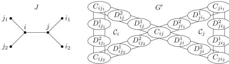
Fig. 2 A part of the construction of G' for s = 2 . Cliques C_{ab} representing edge sets E_{ab} \subseteq E(G) are connected through secondary cliques D_{ab}^p
