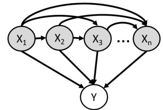
Discriminative (logistic regression)
