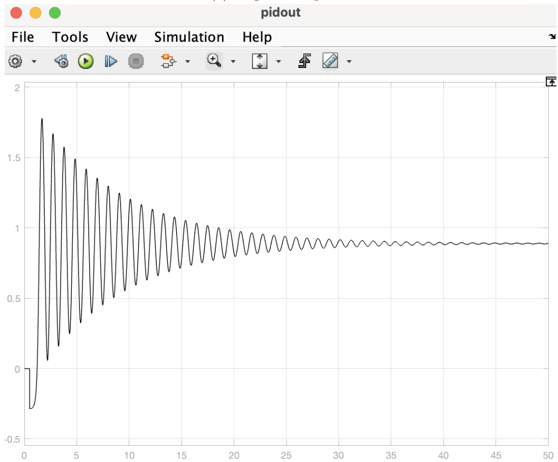
(b) PID Output Response
