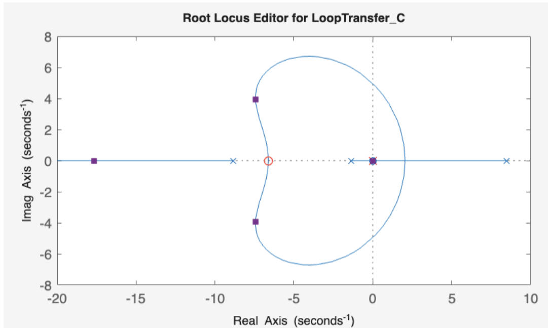
(b) Root Locus plot with Controller
