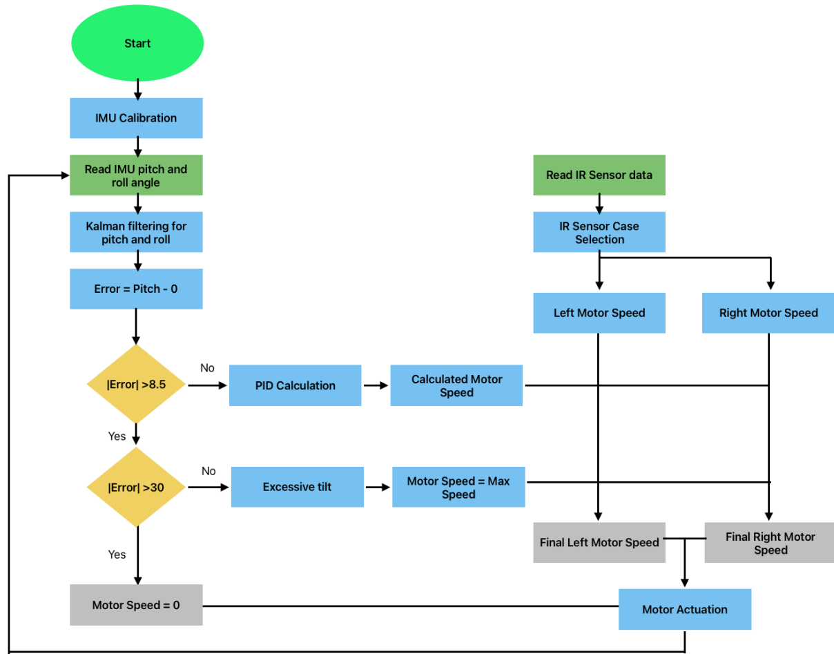
Figure 28: Code Overview flowchart
