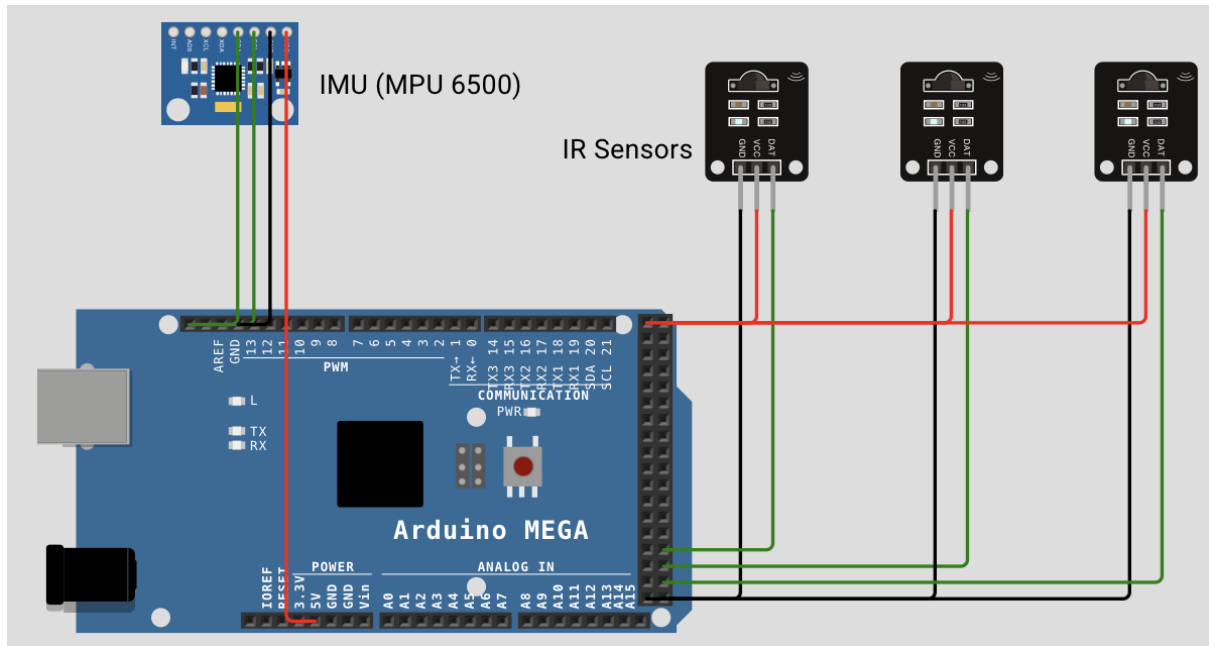
Figure 18: Sensor connections
