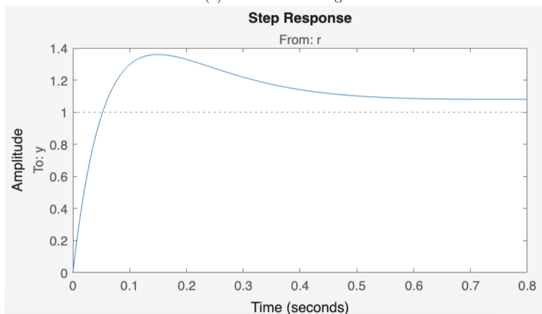
(b) Step Response with Controller
