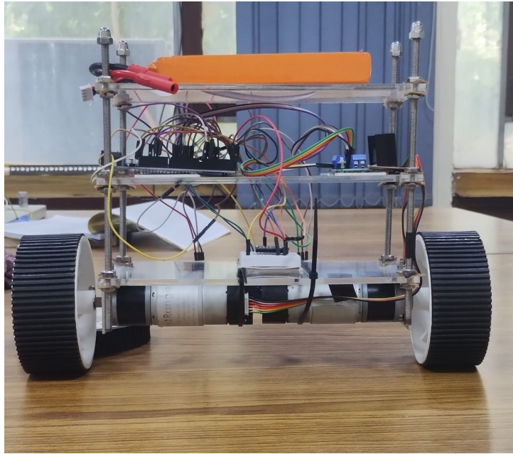
Figure 2: Back View
