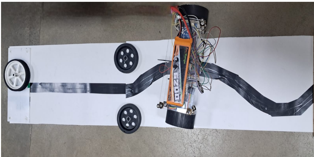
Figure 20: Top View
