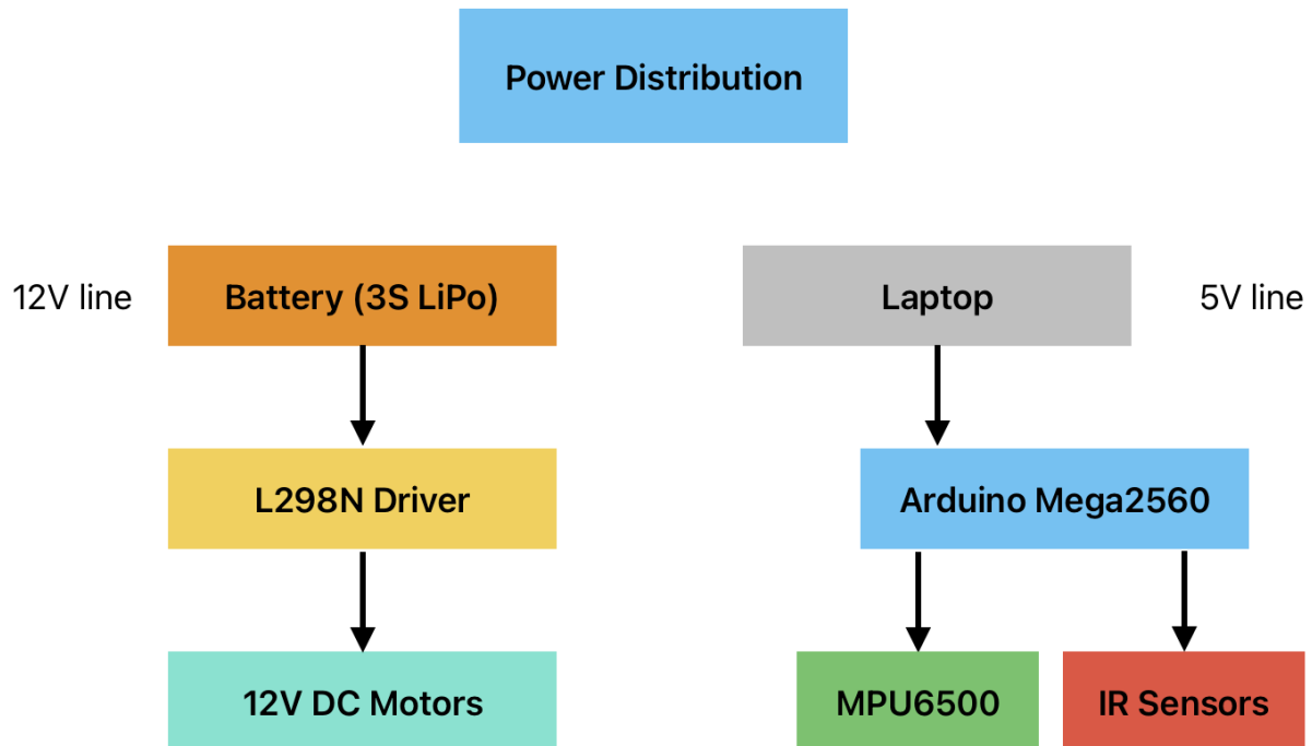
Figure 16: Power Distribution flowchart
