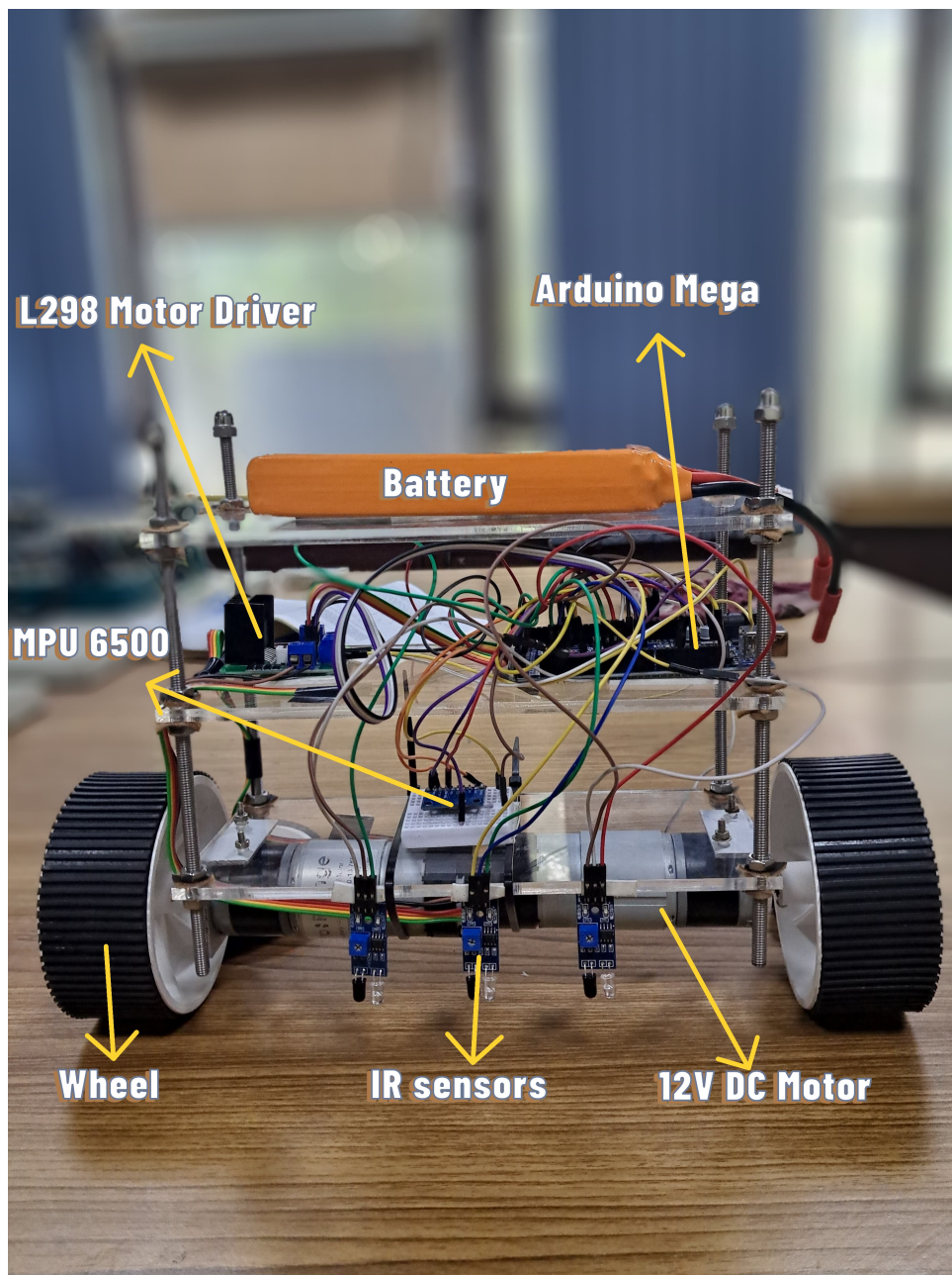
Figure 1: Front View
