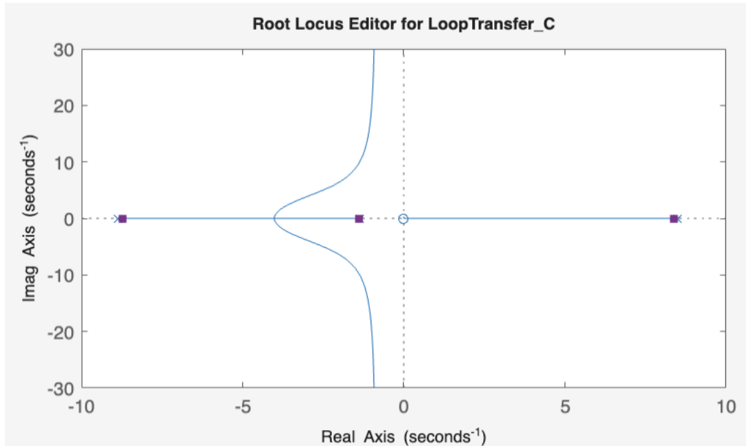
(a) Root Locus plot of Plant
