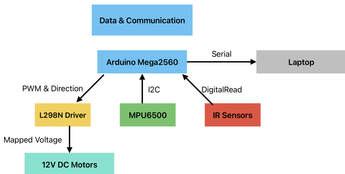
Figure 17: Data flow path
