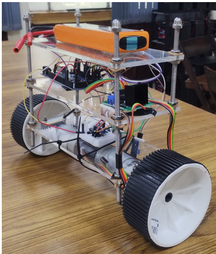
Figure 3: Isometric View
