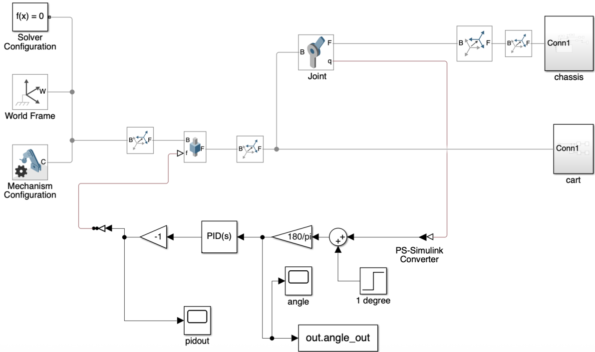
(a) Simulink modelling
