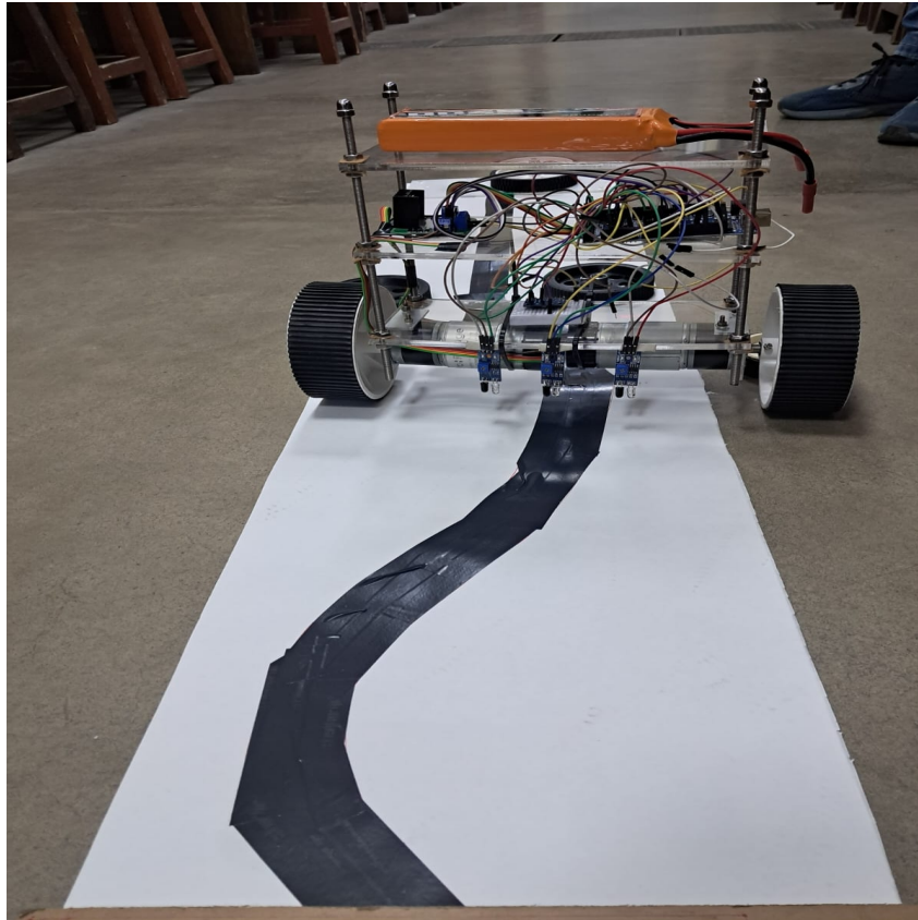
Figure 19: Front View
