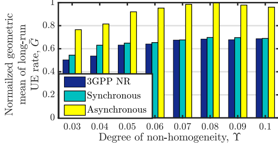
Figure 13: Comparison of normalized \bar{G} for M = 100 non-homogeneously distributed UE achieved with 3GPP NR, synchronous and asynchronous schemes.
