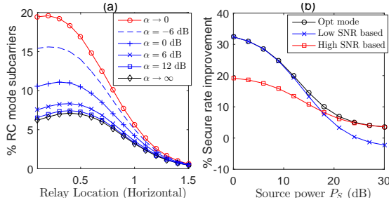
Fig. 1: (a) Performance with horizontal variation in relay position, (b) Secure rate improvement through mode selection.
