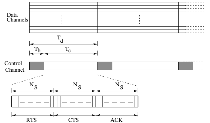
Fig. 1. MAC frame structure
