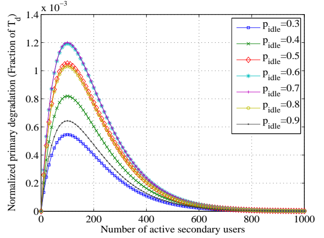
Fig. 10. Expected PU degradation with N_T = 30 and N_S = 100
