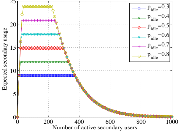
Fig. 9. Average secondary usage with N_T = 30 and N_S = 100
