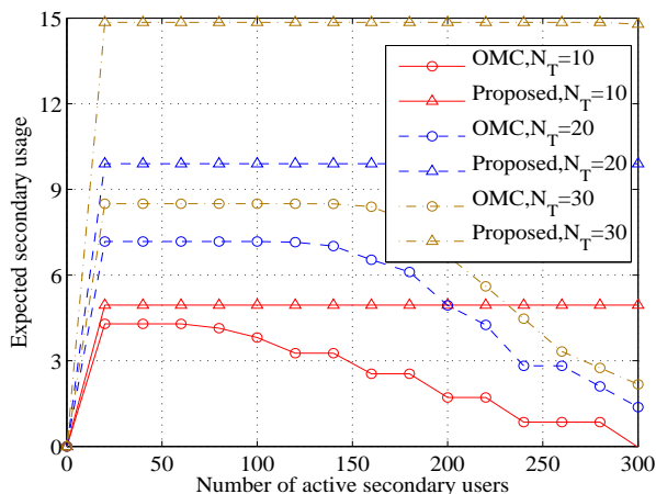
Fig. 16. Expected secondary usage comparison with OMC-MAC with p_{idle} = 0.5 and N_S = 100 .
