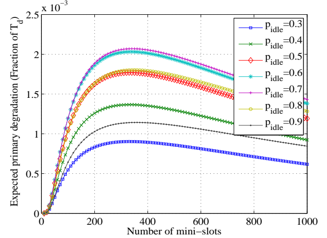
Fig. 11. Expected PU degradation with N_T = 30 and \Lambda = 100
