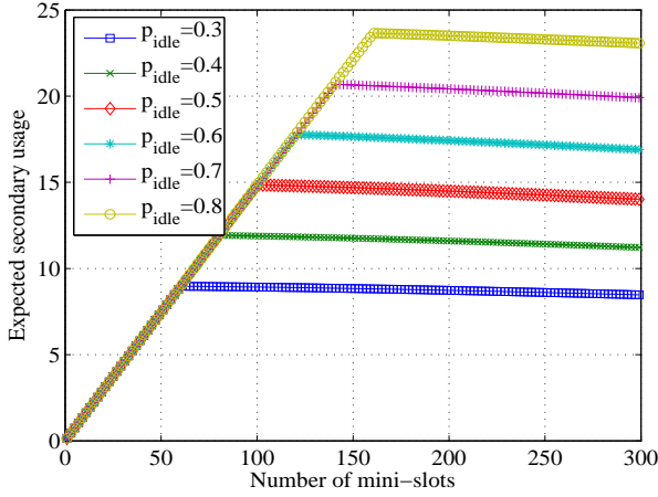
Fig. 8. Average secondary usage with N_T = 30 and \lambda_s = 3
