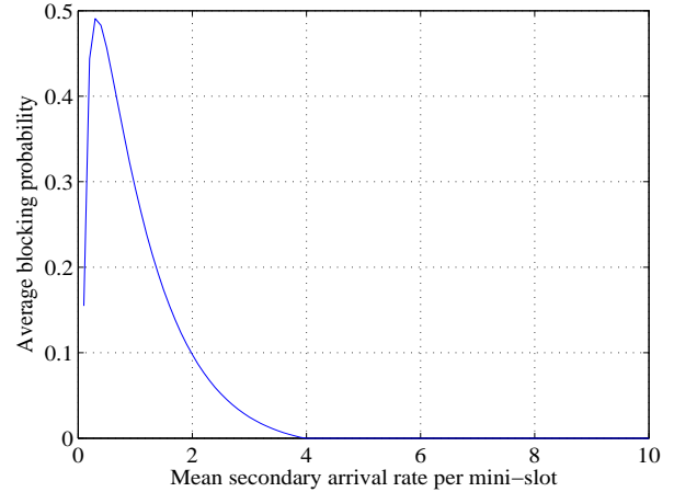
Fig. 6. Average blocking probability with N_T = 30 , N_S = 200 , p_{idle} = 0.5
